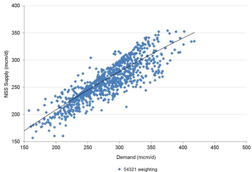
Figure 1 – Non storage supply (NSS) versus demand for the winters 2014/15 to 2018/19
