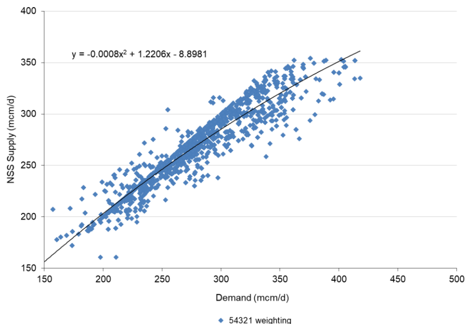
Figure 1 – Non storage supply (NSS) versus demand for the winters 2017/18 to 2021/22
