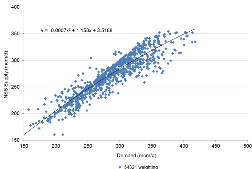
Figure 1 – Non storage supply (NSS) versus demand for the winters 2016/17 to 2020/21
