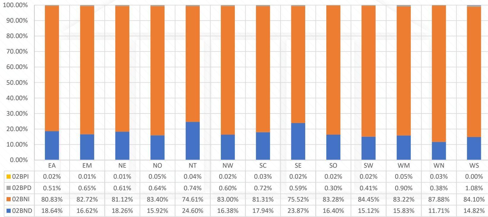
GasYr 2019 02B AQ Change - excl SIUs
