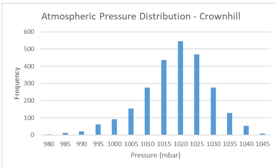
Figure 8: Atmospheric Pressure Distribution for Crownhill
