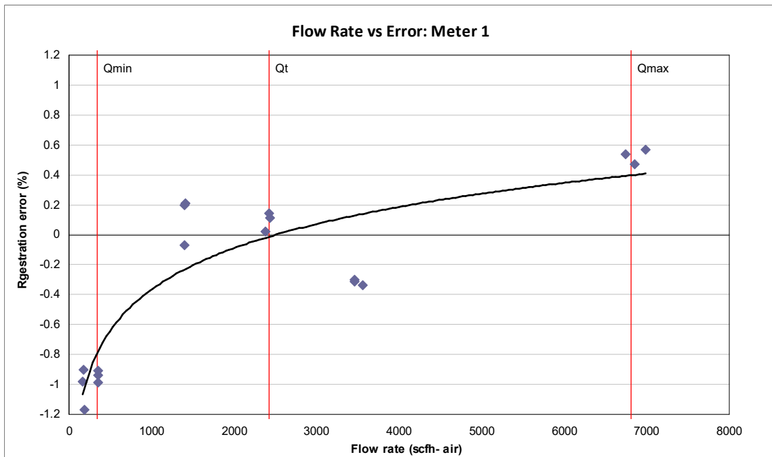
Figure 21: Typical Calibration Curve for an RPD Meter
