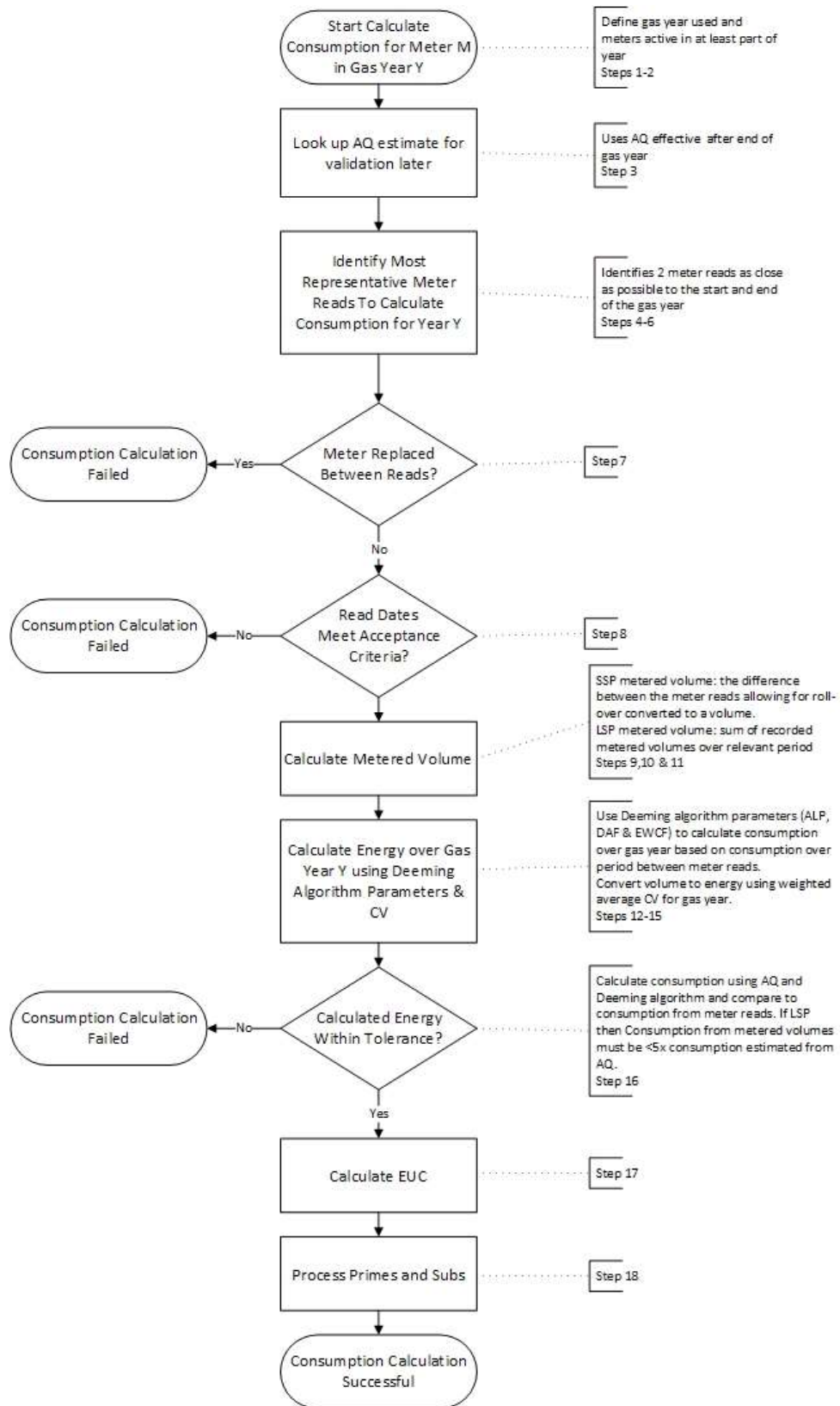
Figure 16: Consumption Algorithm Flow Chart
