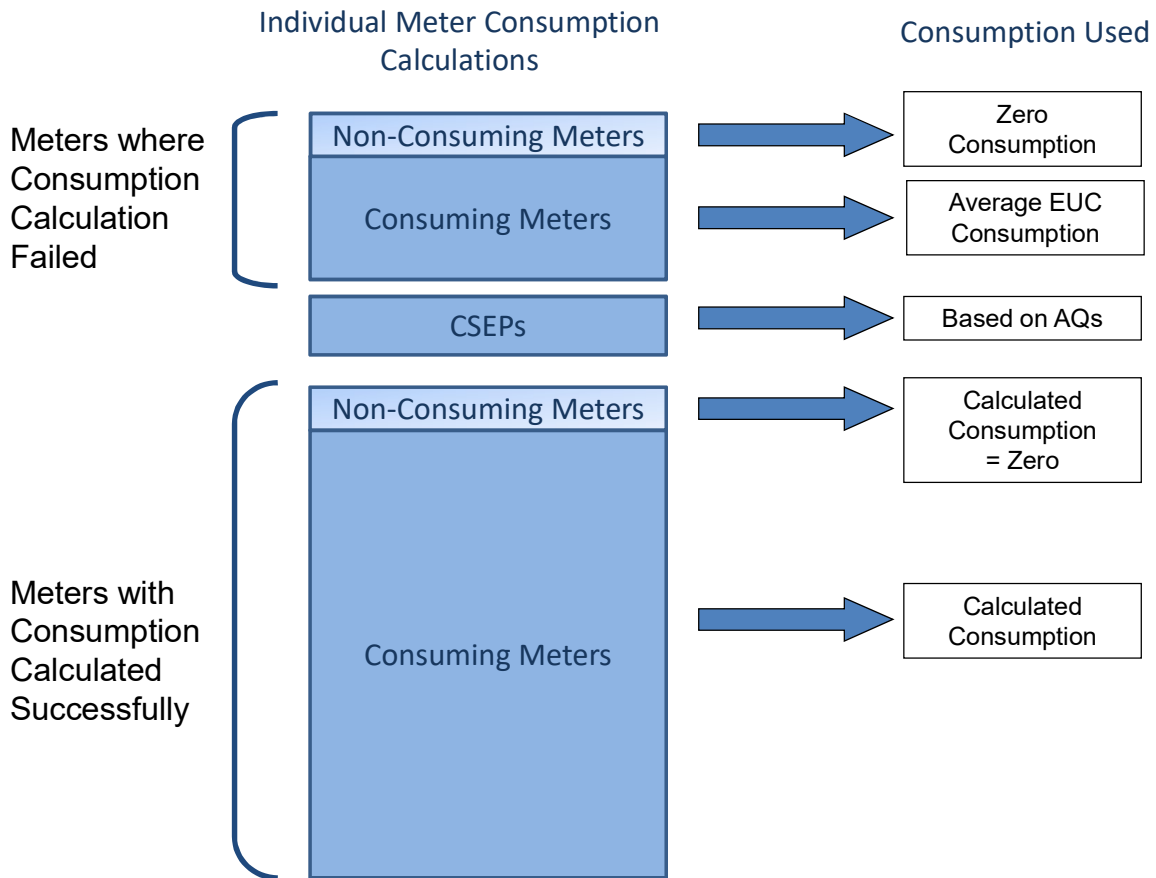
Figure 18: Consumption Method used for each type of Meter Point
