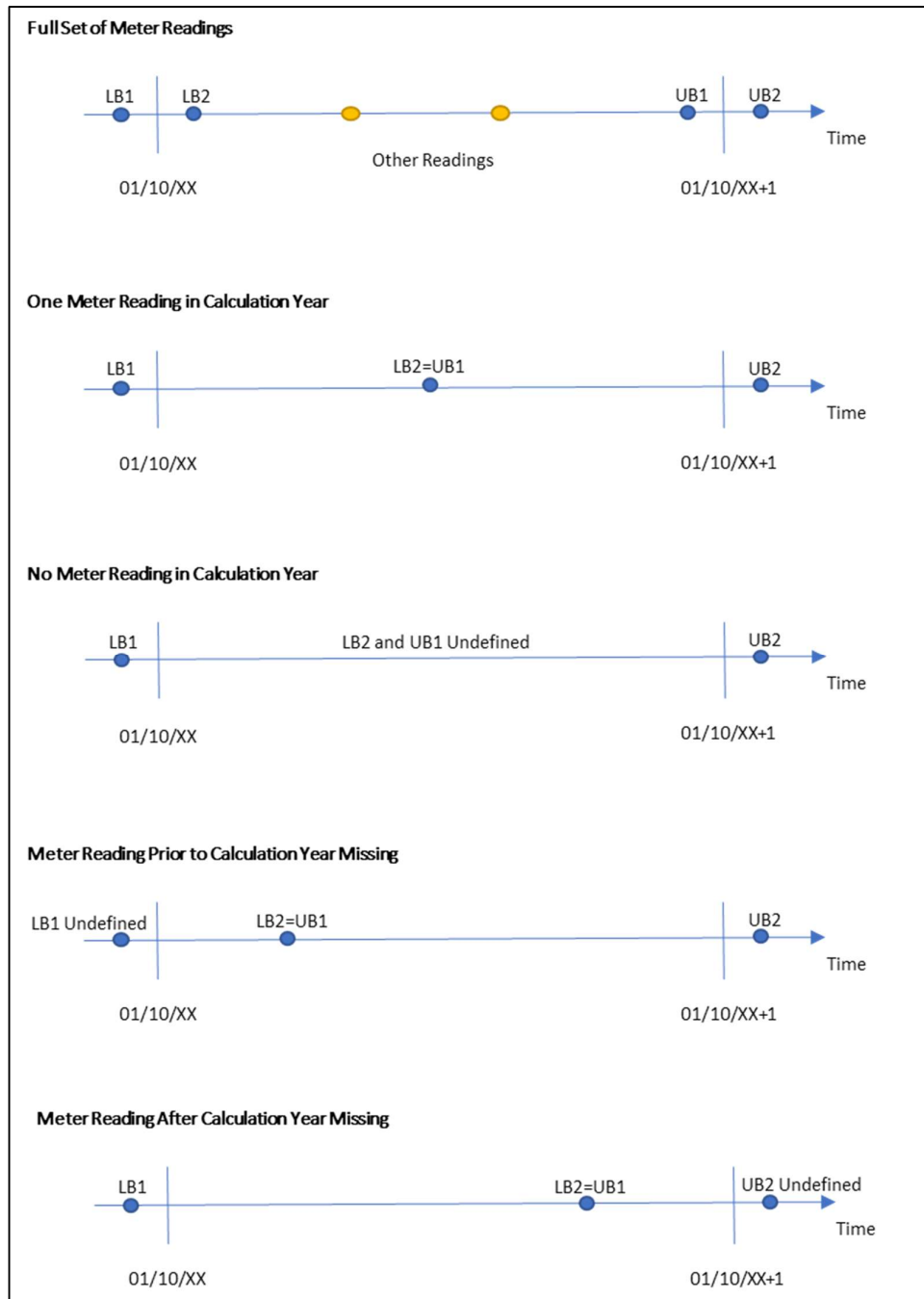
Figure 17: Meter Read Availability Scenarios
